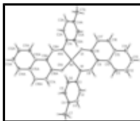
Fig. 1. The molecular structure of (I). Displacement ellipsoids are drawn at the 30% probability level (symmetry code (A): -x+2, -y, -z ).
